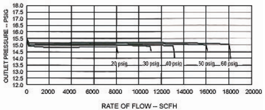
Performance Curves
