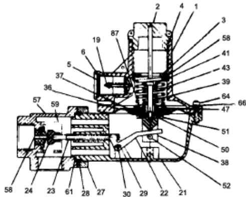
CL34-2 Pilot Reference Schematic (see main parts list Item 71B for pilot subassemblies)
