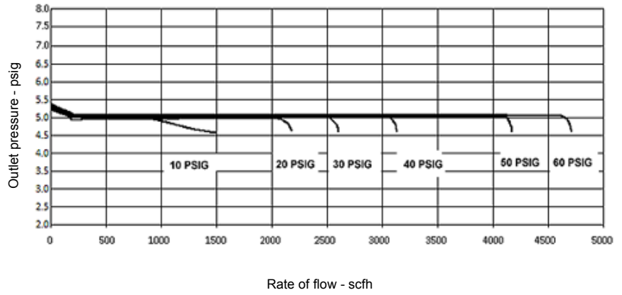
CL-31 Performance Curves 5 PSIG Set Point
