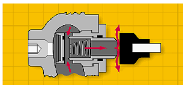
A. Standard regulator and upstream monitor orifice.
