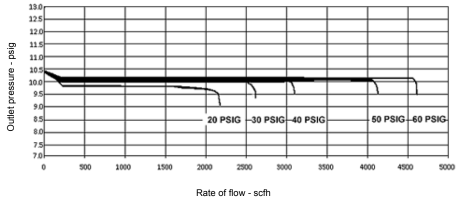
CL-31 Performance Curves 10 PSIG Set Point
