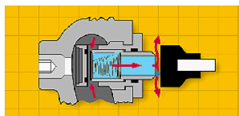
B. Standard regulator orifice failed; upstream monitor orifice control.
