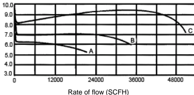
B838 Relief Curves
