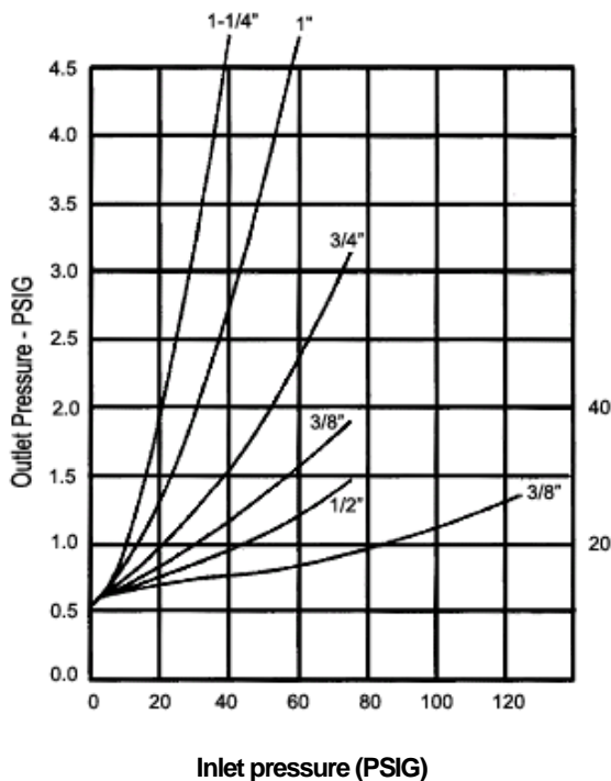
B838 Relief Curves
