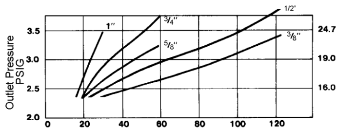
Relief Valve Characteristics 1
