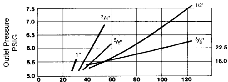
Relief Valve Characteristics 1
