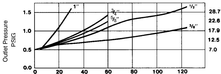
Relief Valve Characteristics 1
